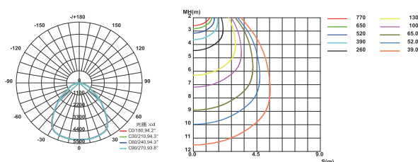
Light Distribution Curve
